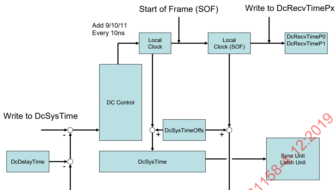
Figure 48 – Distributed clock
