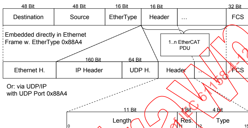
Figure 3 – Frame structure
