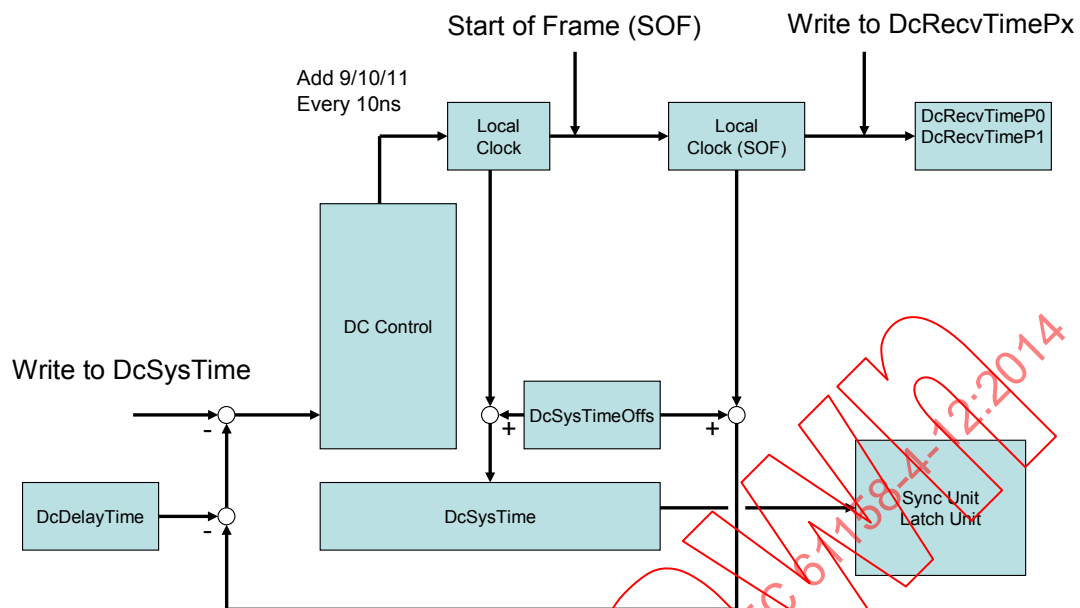
Figure 48 – Distributed clock
