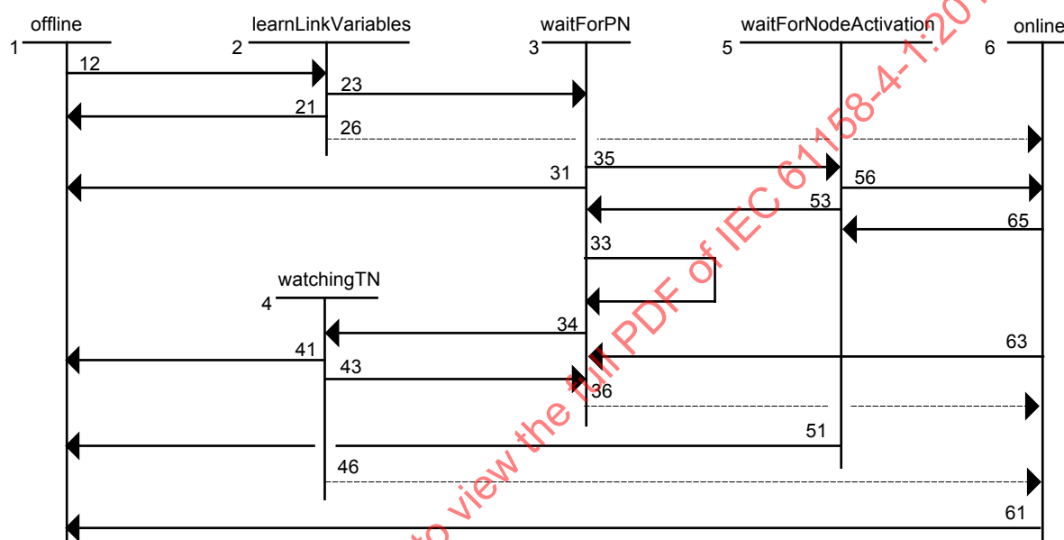
DLE-state FSM
