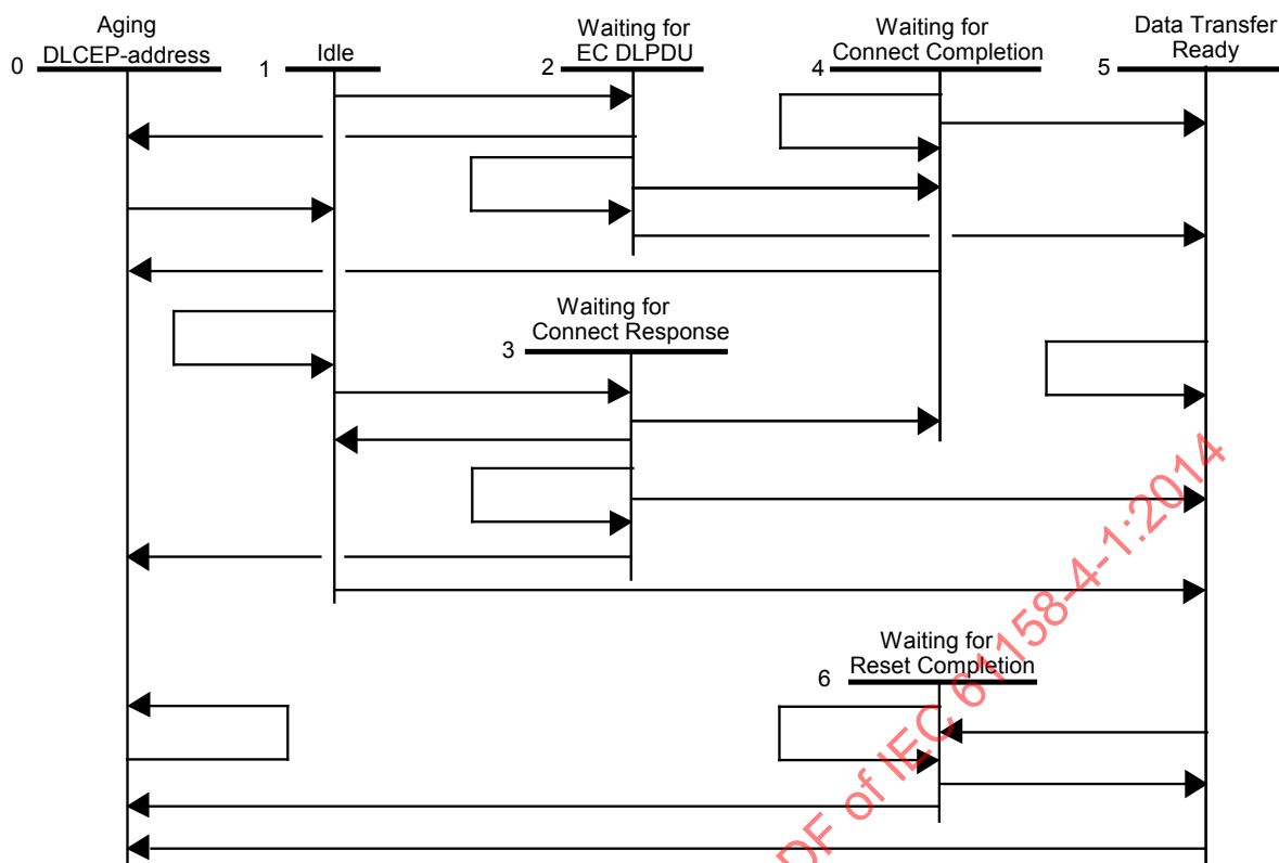
Figure 11 – State transition diagram for a DLCEP
