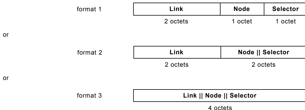
Figure 8 – DL-address alternative structures
