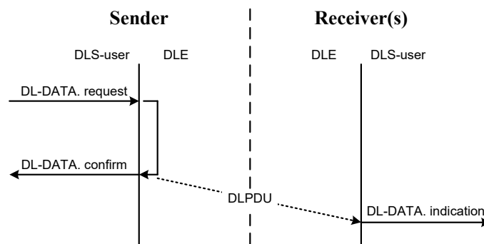
Figure 2 – Sequence diagram of DL-DATA service
