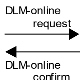
Figure 23 – Sequence of primitives for a DLM-online request
