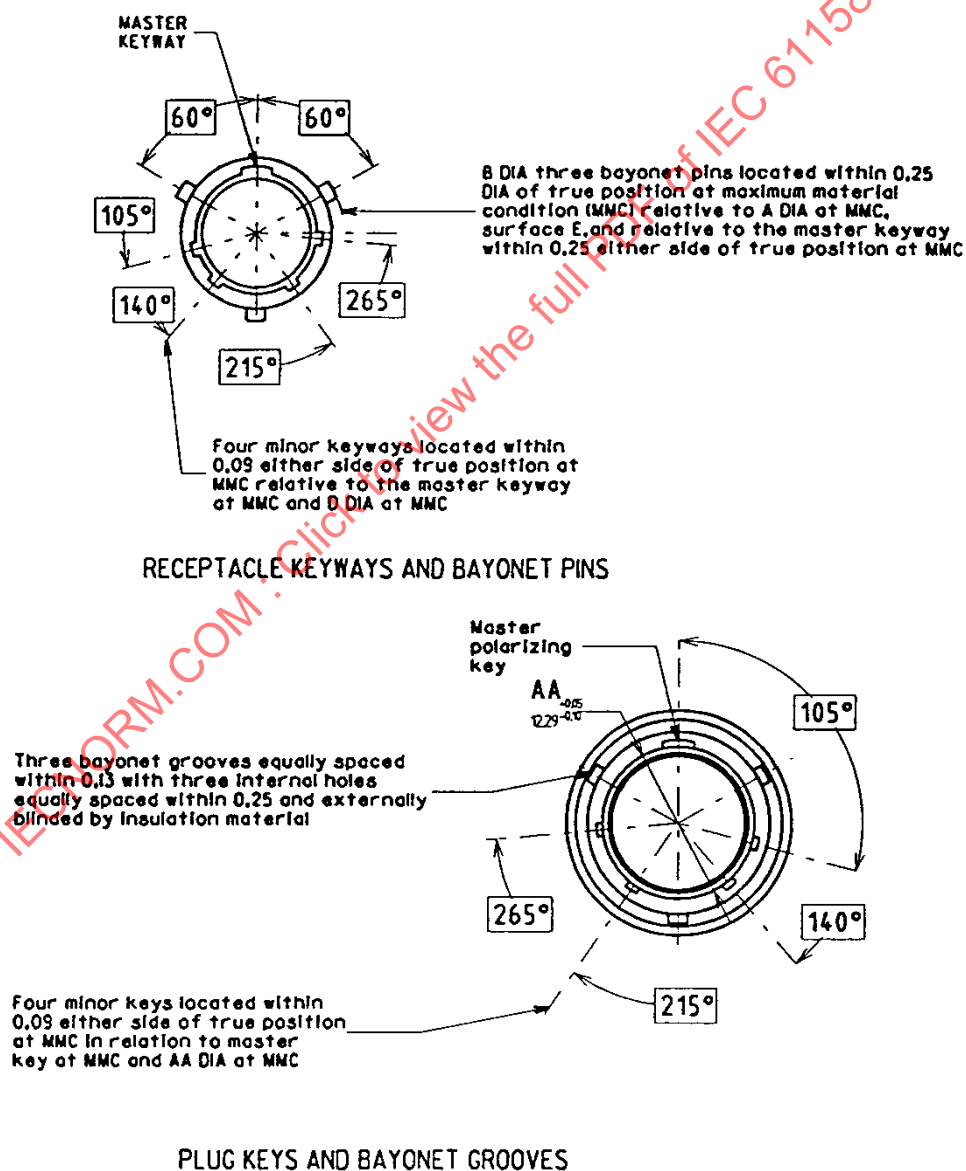
Figure A.3 – External fieldbus connector keyways, keys, and bayonet pins and grooves
