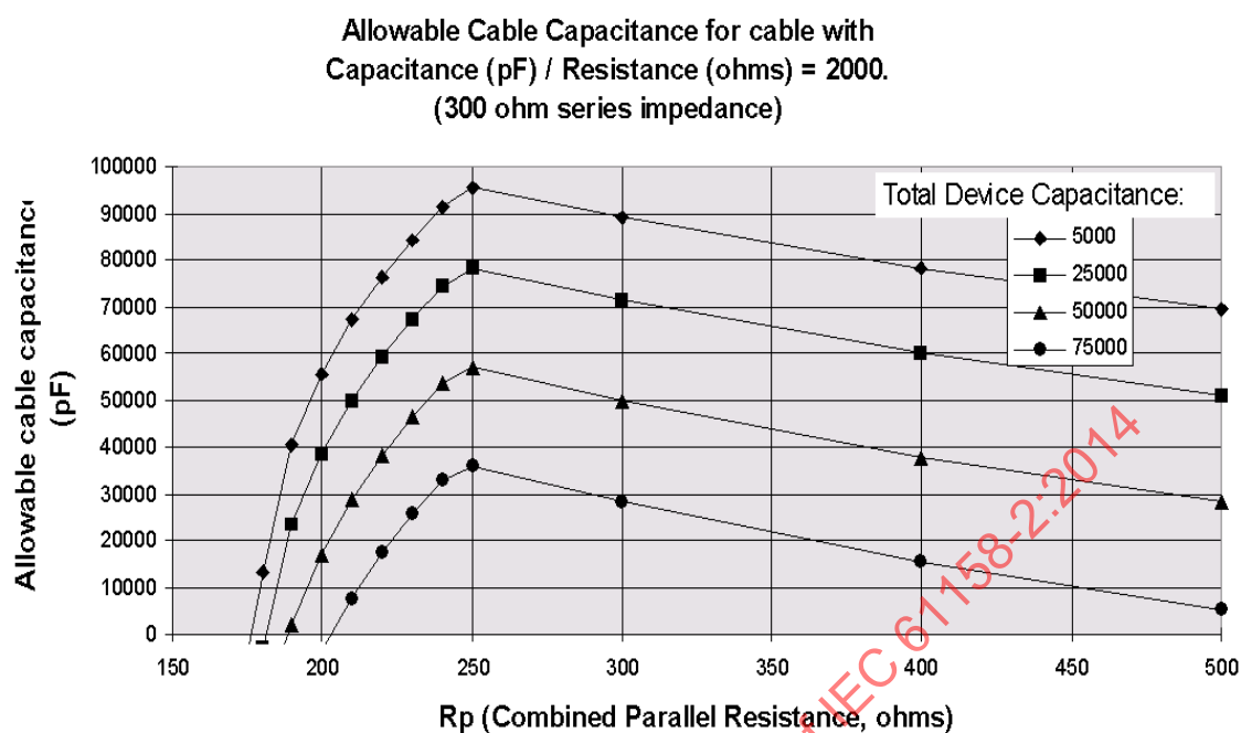
Figure T.18 – Cable capacitance for C_{cbl}/R_{cbl}=2\ 000 , 300 \Omega series resistance
