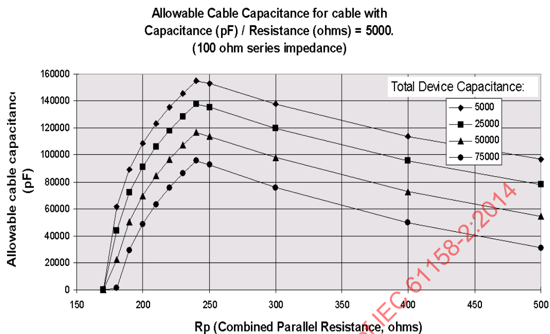
Figure T.20 – Cable capacitance for C_{cbl}/R_{cbl}=5000 , 100 \Omega series resistance
