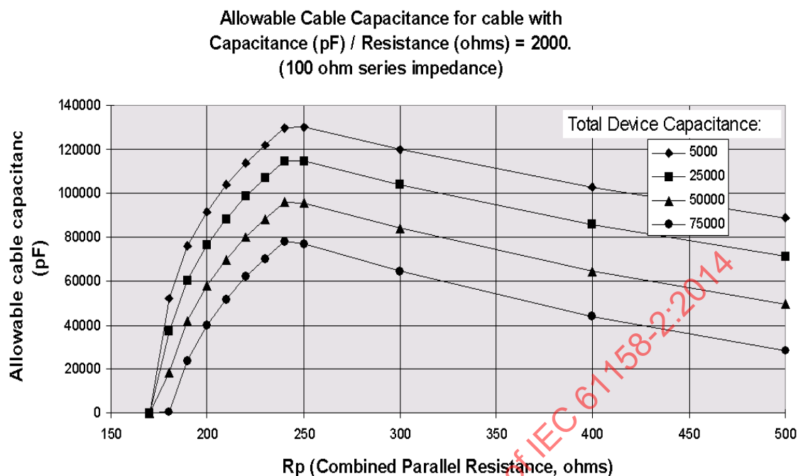
Figure T.16 – Cable capacitance for C_{cbl}/R_{cbl}=2\ 000 , 100 \Omega series resistance
