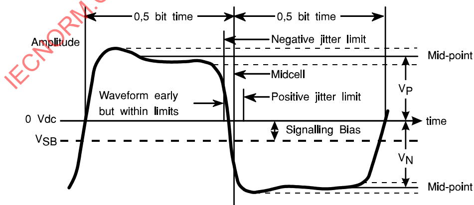
Figure 73 – Transmitted and received bit cell jitter (zero crossing point deviation)
