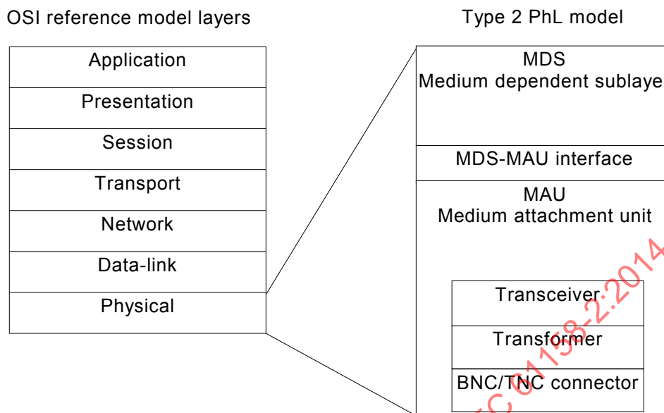
Figure 76 – Components of 5 Mbit/s, voltage-mode, coaxial wire PhL variant
