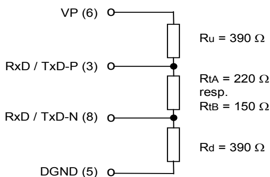
Figure 101 – Bus terminator
