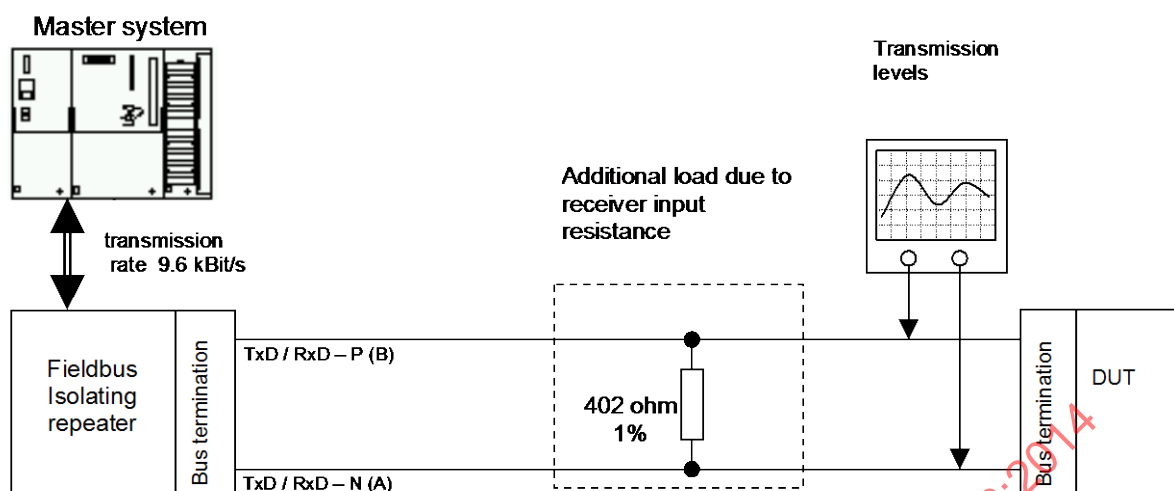
Figure 108 – Test set-up for measurement of the transmission levels
