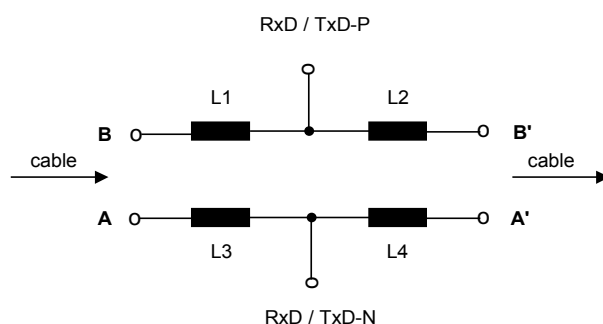
Figure 99 – Example for a connector with integrated inductance
