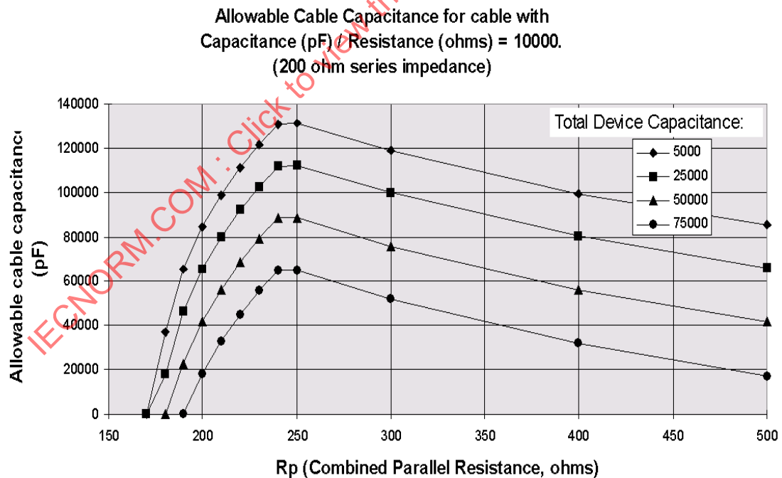
Figure T.25 – Cable capacitance for C_{cbl}/R_{cbl}=10\ 000 , 200 \Omega series resistance
