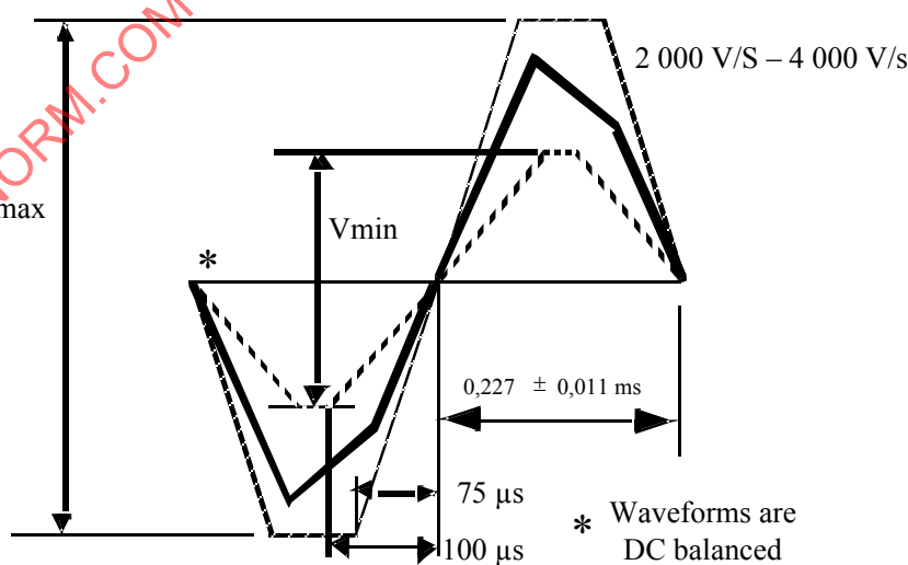
2 200 Hz transmit waveform limits
