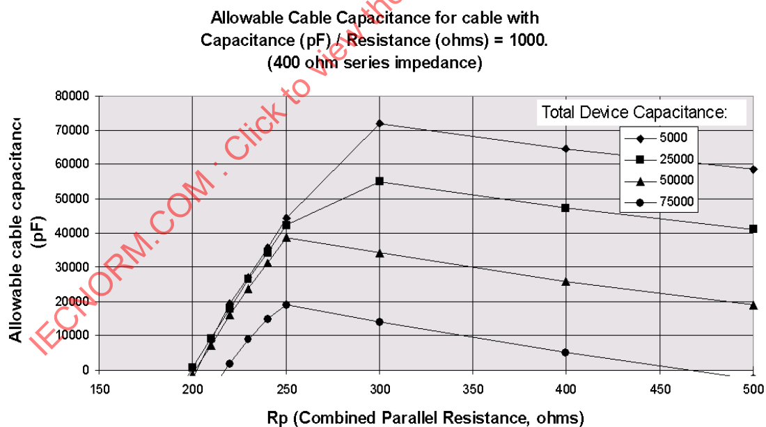
Figure T.15 – Cable capacitance for C_{cbl}/R_{cbl}=1\ 000 , 400 \Omega series resistance
