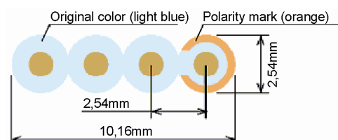
Figure R.4 – PhL-P flat cable cross section – without key
