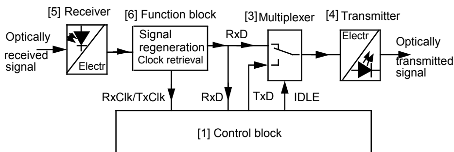
Figure 133 – Functions of a slave connection
