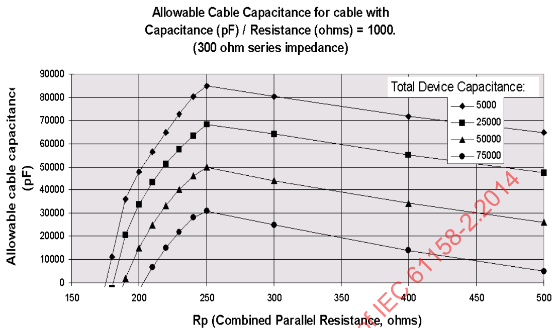
Figure T.14 – Cable capacitance for C_{cbl}/R_{cbl}=1\ 000 , 300 \Omega series resistance
