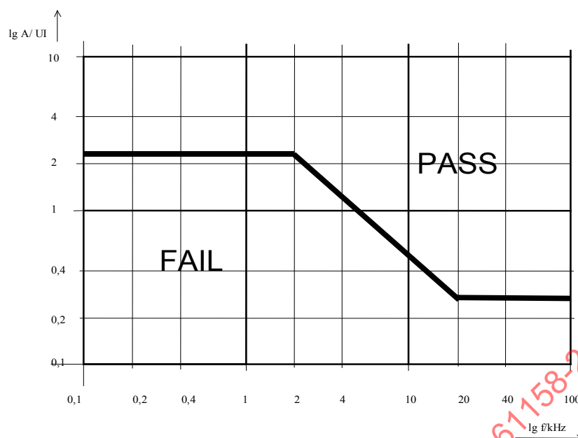
Figure 55 – Jitter tolerance
