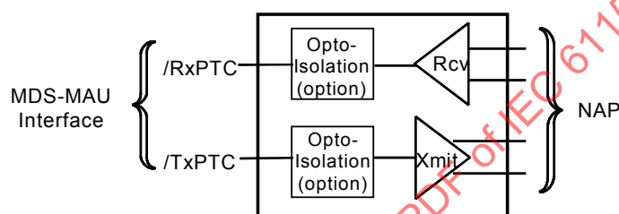
Figure 89 – NAP transceiver
