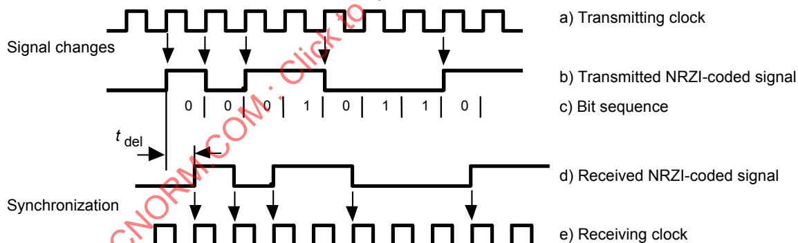
Figure 52 – Example of an NRZI-coded signal
