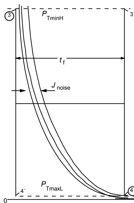
Figure 128 – Display of jitter ( J_{\text{noise}} )
