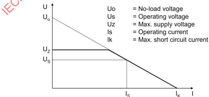
Figure 96 – Output characteristic curve of a power supply of the category EEx ia
