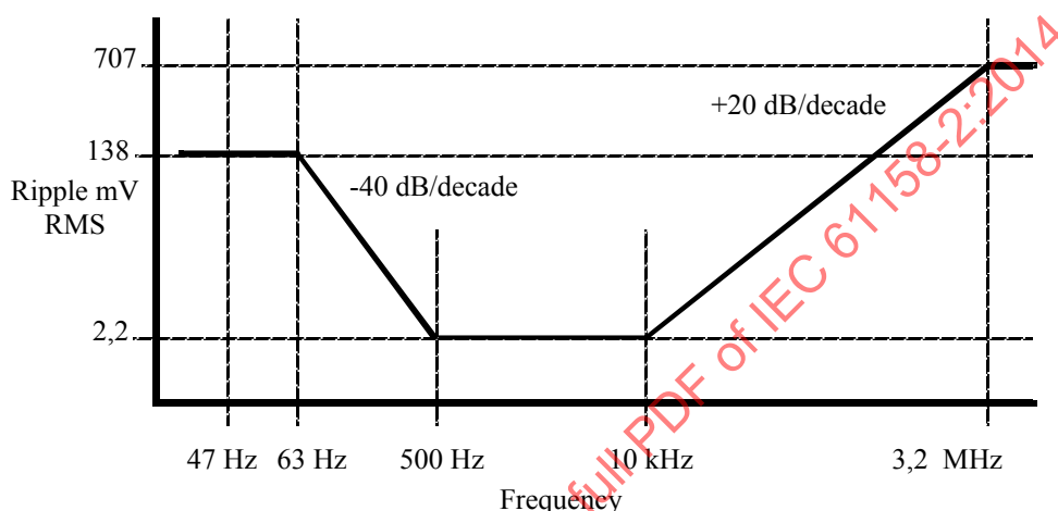
Figure 170 – Network power supply ripple
