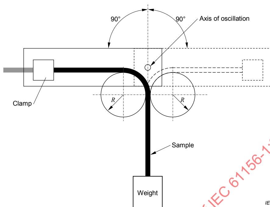
Figure 16 – Repeated bending test configuration
