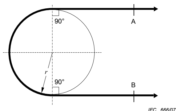
Figure 14 – U-bend test configuration
