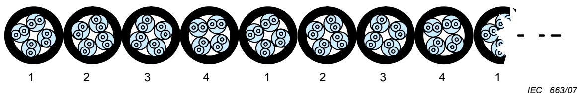
Figure 11 – Test assembly cross-section; four parallel cables
