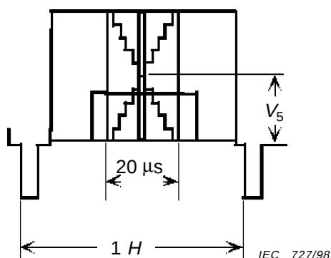
Figure 4 – Waveform of a horizontal line for \bar{B} = 77 \%
