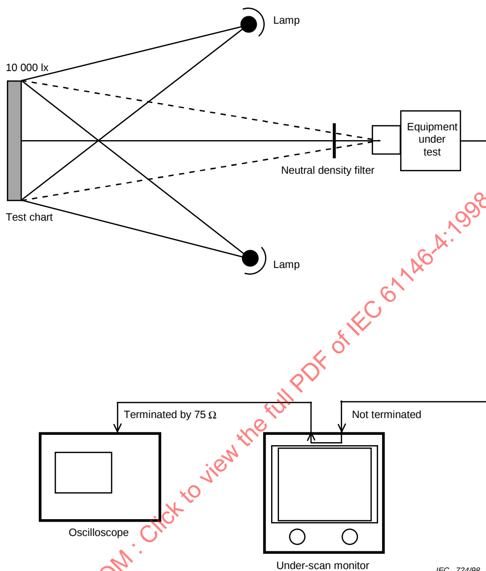
Figure 1 – Equipment arrangement for measurement of dependency on illumination level
