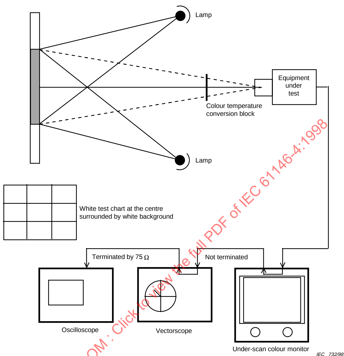
Figure 9 – Equipment arrangement for measurement of automatic white balance
