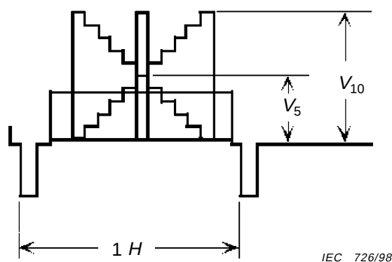
Figure 3 – Waveform of a horizontal line for \bar{B} = 27 \%
