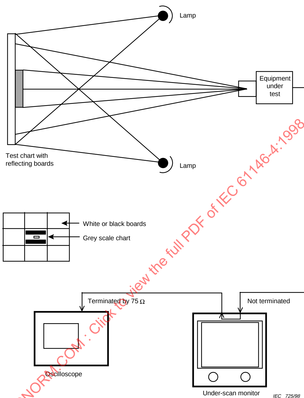
Figure 2 – Equipment arrangement for measurement of dependency on average brightness
