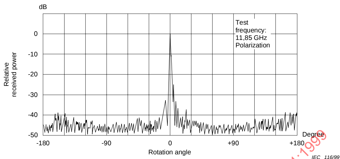
Figure 9a – Wide-angle radiation pattern
