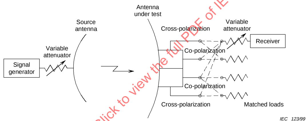
Figure 12b – Multiple-beam antenna
