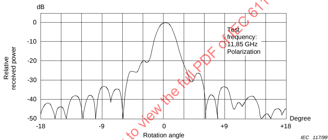
Figure 9b – Near-beam axis radiation pattern
