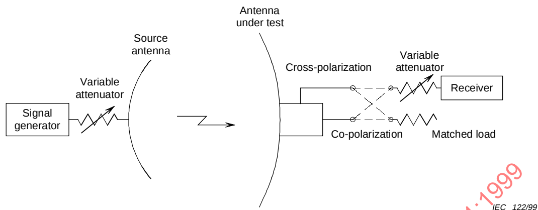
Figure 12a – Single-beam antenna
