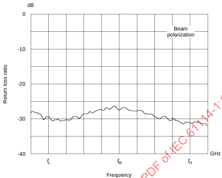
Figure 7 – Impedance matching graphical presentation
