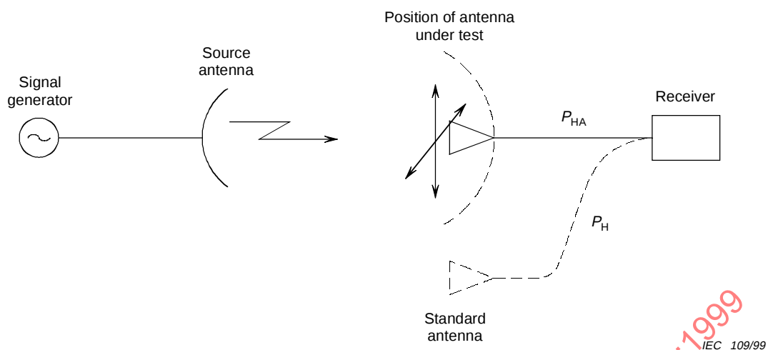
Figure 2 – Field intensity calibration
