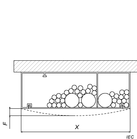
Figure 104a – Rectangular or similar cross section CTS/CDS
