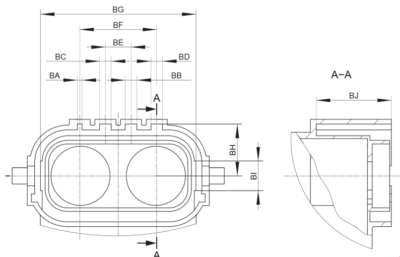
Figure 4 – Free connector codings
