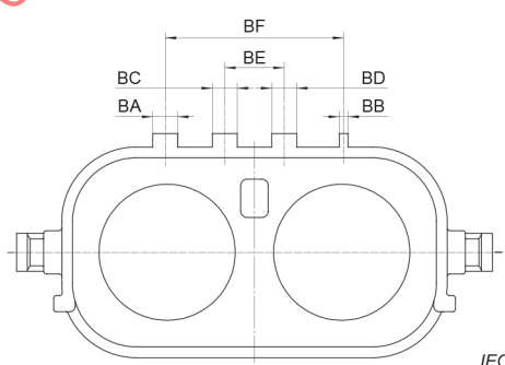
Figure 6 – Fixed connector codings
