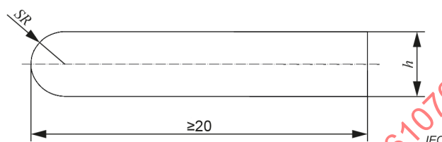
Figure 8 – Gauge for power contacts
