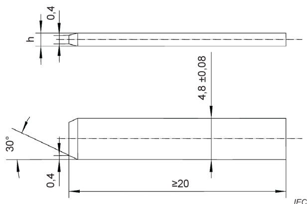
Figure 10 – Gauge for power contact
