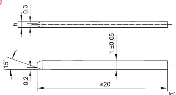
Figure 9 – Gauge for signal contact
