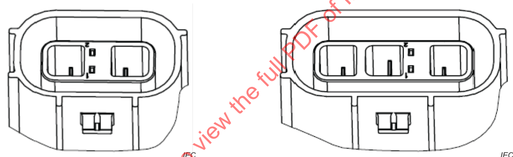
Figure 2 – 2-pole and 3-pole fixed connector
