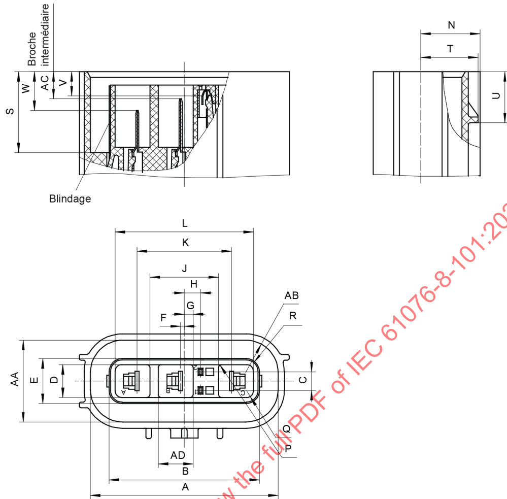
Figure 4 – Embase tripolaire 40 A
