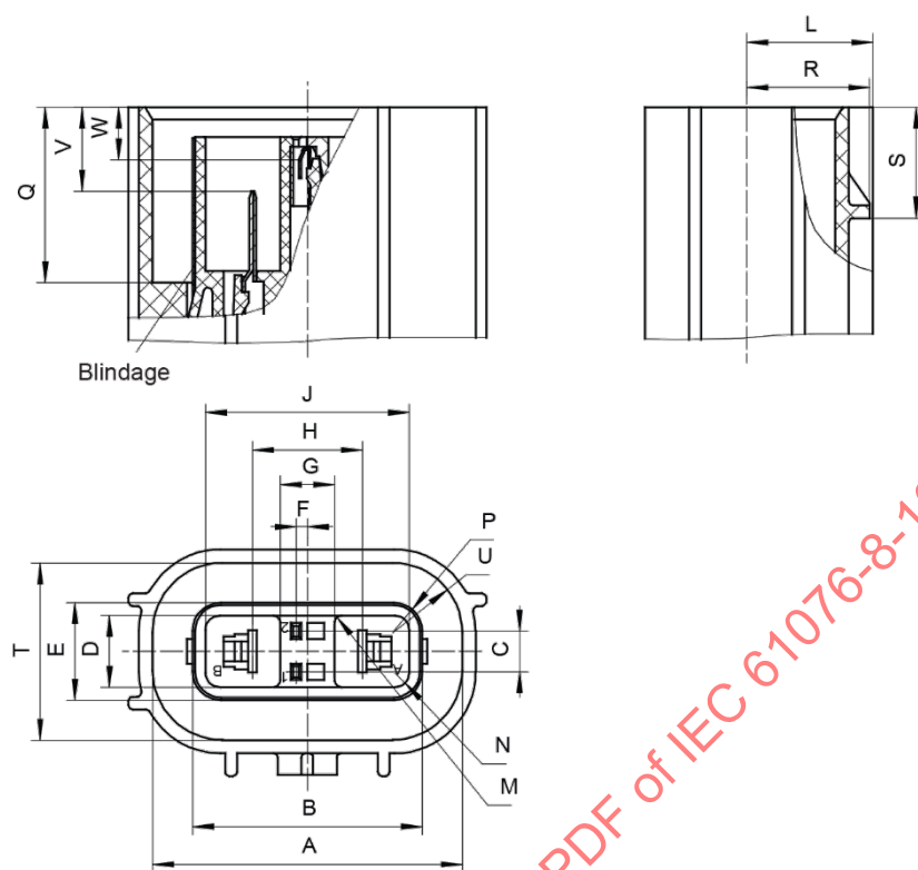
Figure 3 – Embase bipolaire 40 A
