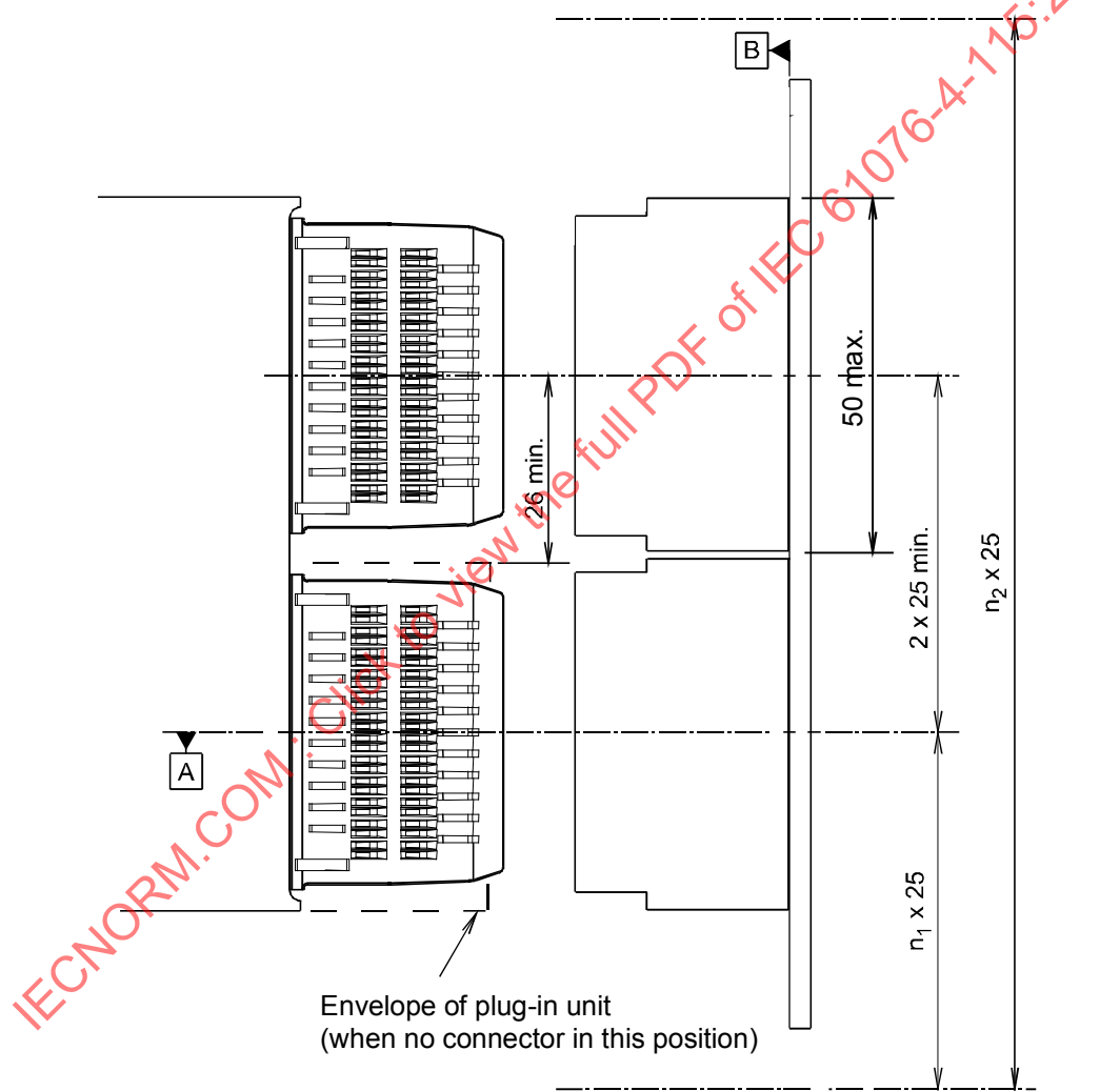
Figure 8 – Height dimensions and mounting pitch
