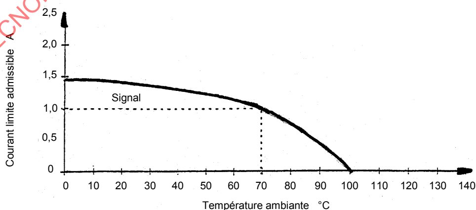
Figure 25 – Courant limite admissible
