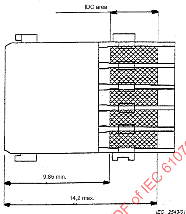
Figure 19 – Free connector terminations
