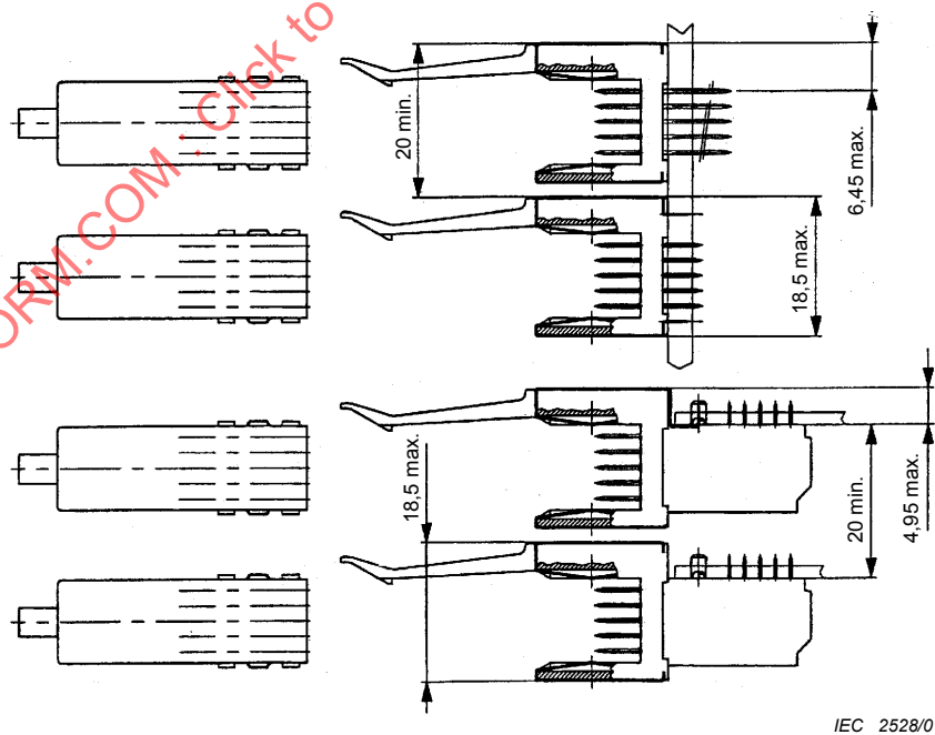
Figure 8 – Width dimensions
