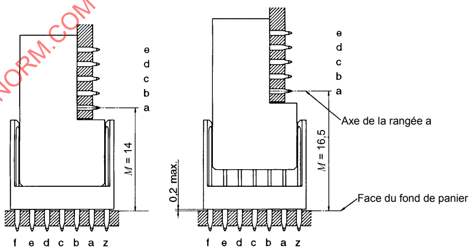
Figure 12 – Plage de contact
