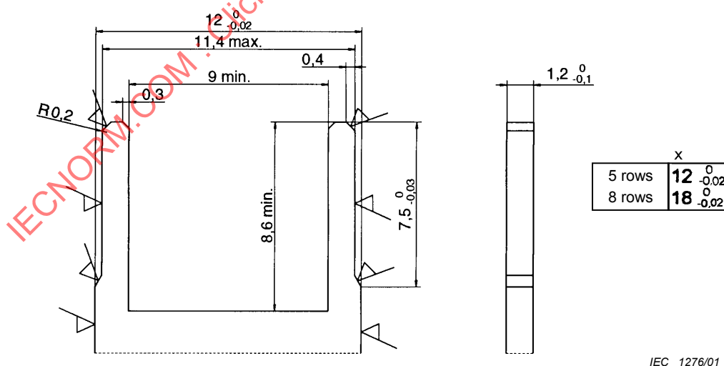
Figure 65 – Sizing and retention force gauges for female contacts
