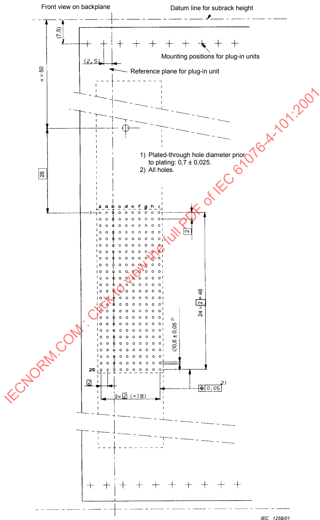
Figure 48 – Hole pattern on backplane for style E
