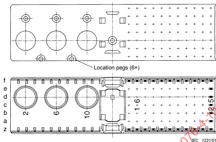
Figure 25 – Dimensions of style M, fixed 50 mm mixed module with three special contacts
