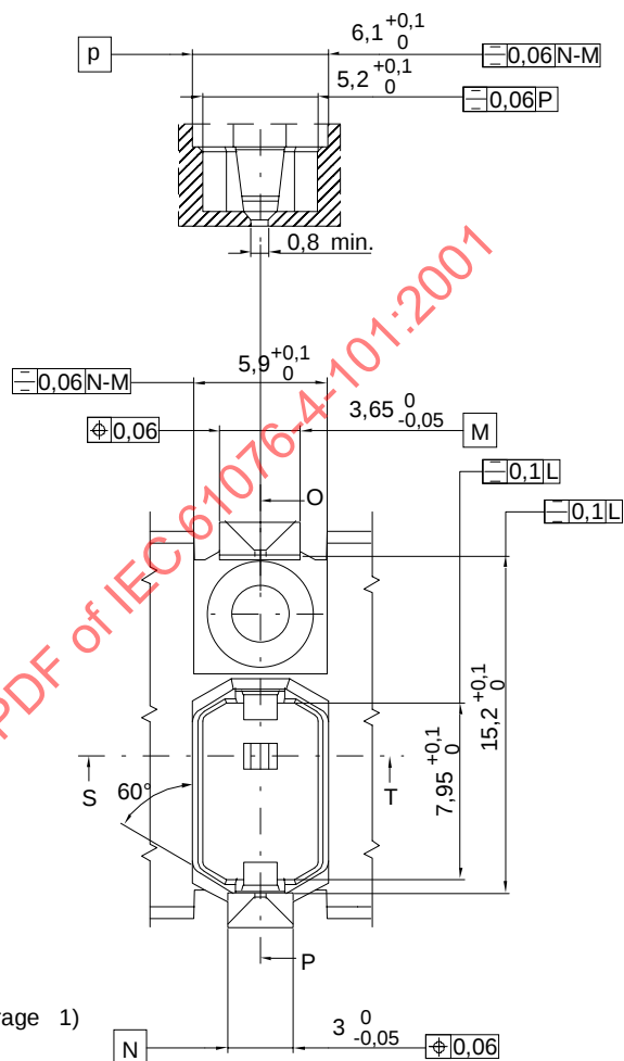
Section ST
