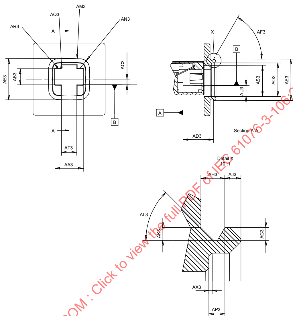
Figure 3 – Embase, Variante 02
