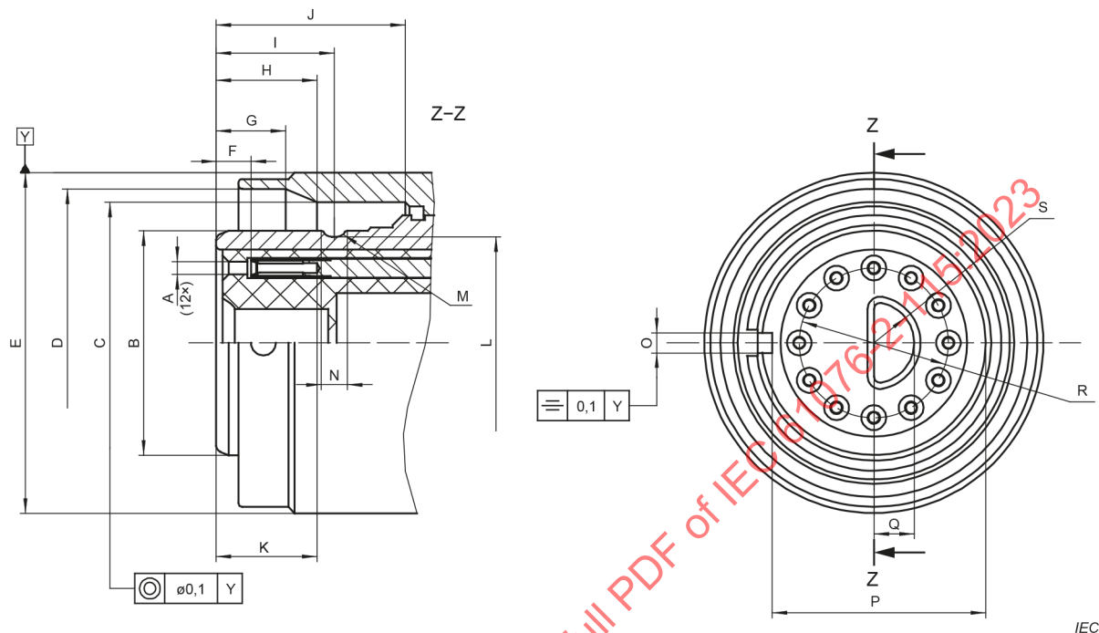
Figure 3 – Free connector
