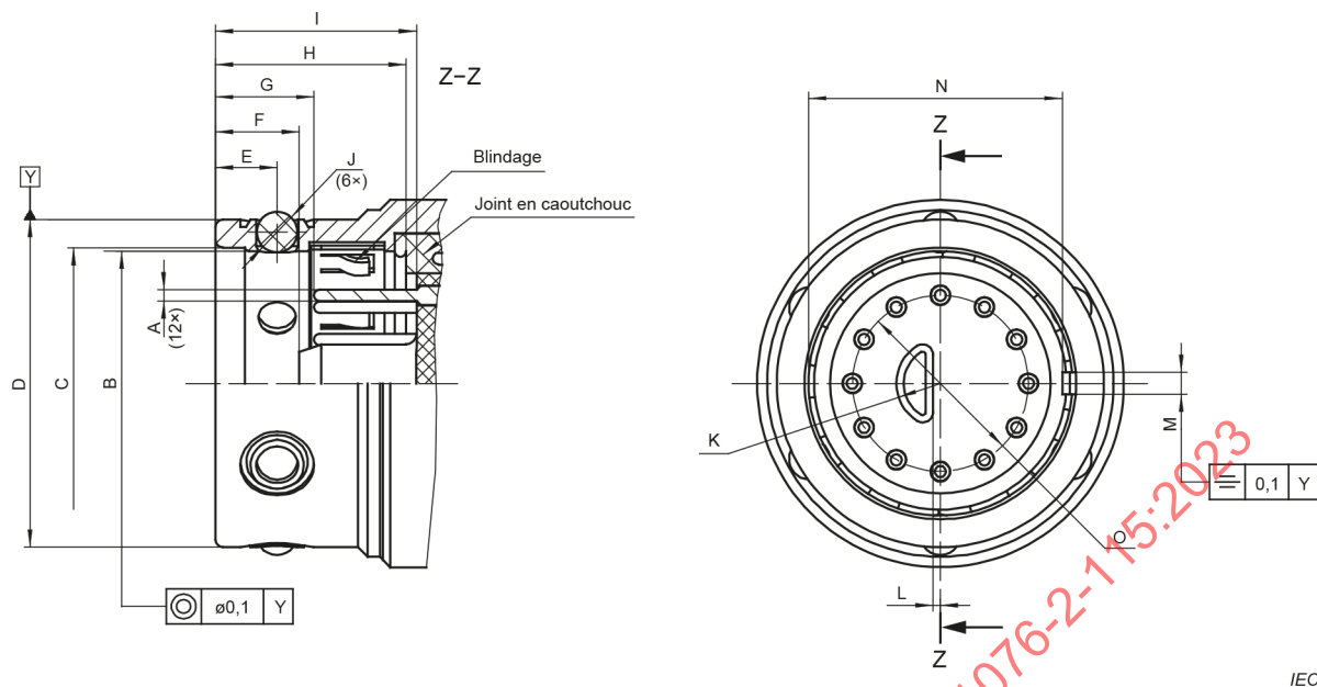
Figure 4 – Embase
