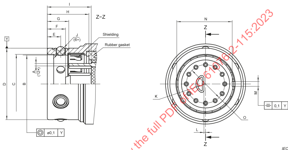
Figure 4 – Fixed connector
