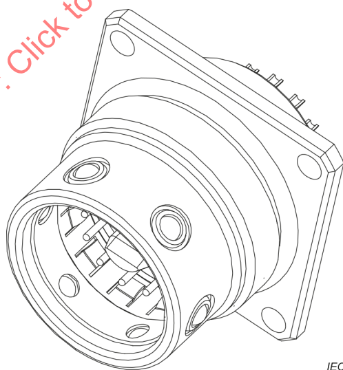
Figure 2 – Fixed connector
