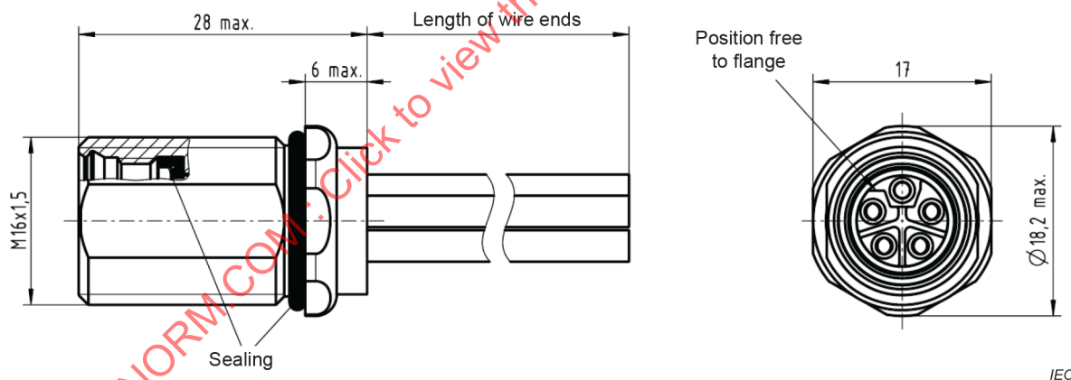
Figure 12 – Fixed connector, female contacts, with M12 screw locking and inner push-pull locking, with wire ends, single hole rear mounting thread M16 × 1,5
