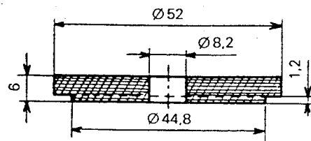
Isolant (A) Insulating material
