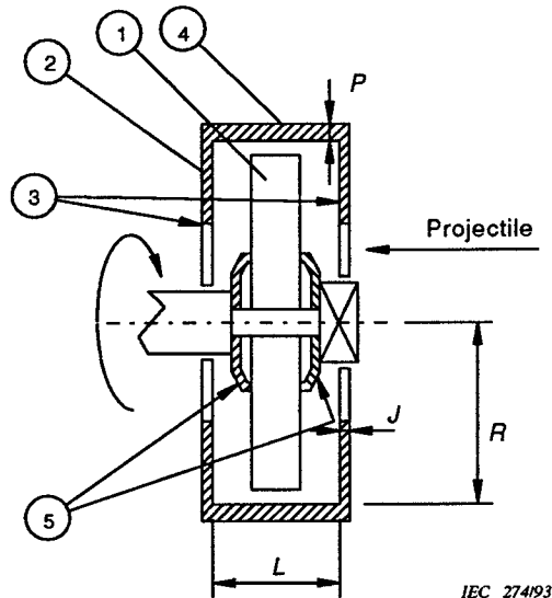
Figure 102 - Schema
