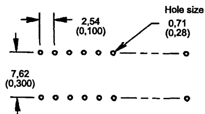
Figure 2 - Mounting dimensions
