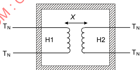
Figure D.3 – Protection of external ACCESSIBLE TERMINALS of two HAZARDOUS LIVE circuits
