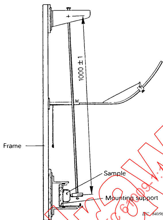
Figure 12 – Mechanical impact test apparatus (9.13.2.1)
