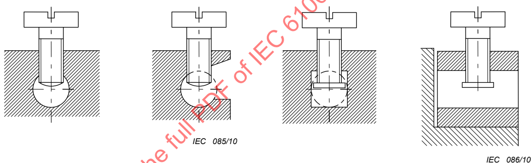
Figure IC.1b – Bornes sans plaque
