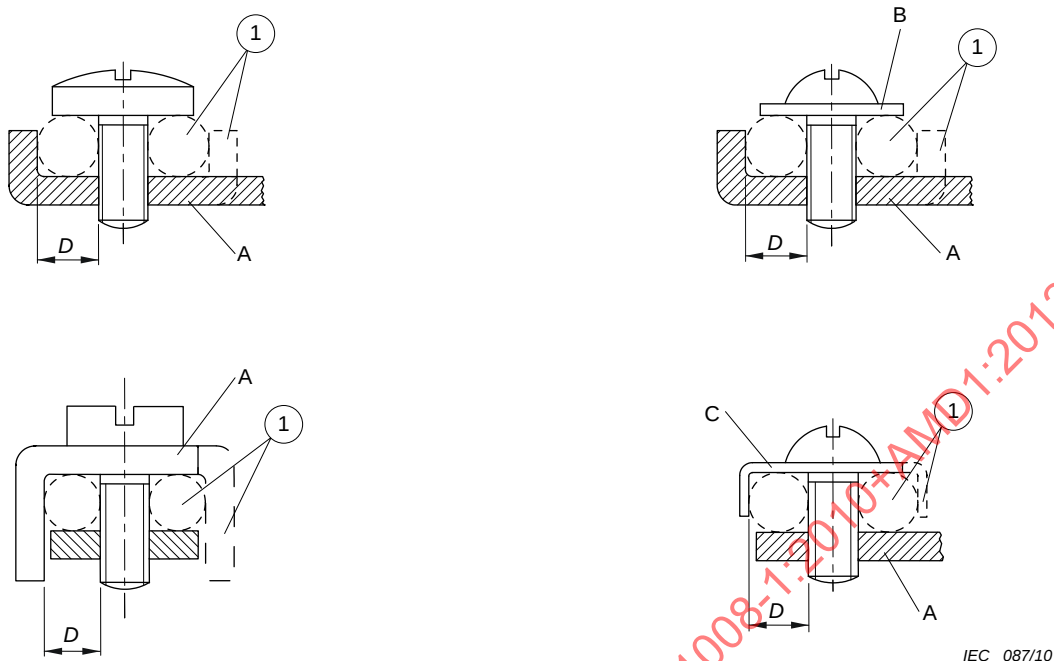
Figure IC.2a – Screw terminals
