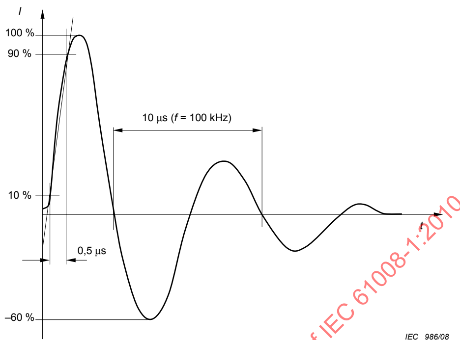
Figure 23 – Current ring wave 0,5 \mu\text{s} /100 kHz
