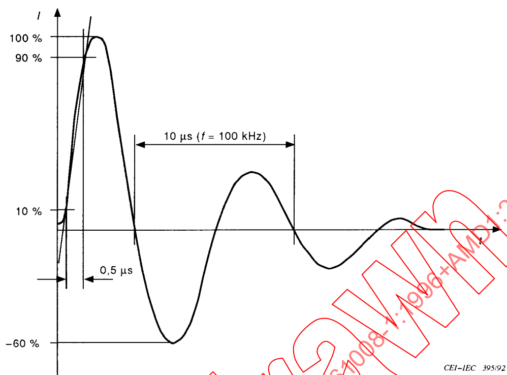
Figure 19a – Current ring wave 0,5 \mu\text{s}/100 \text{ kHz}
