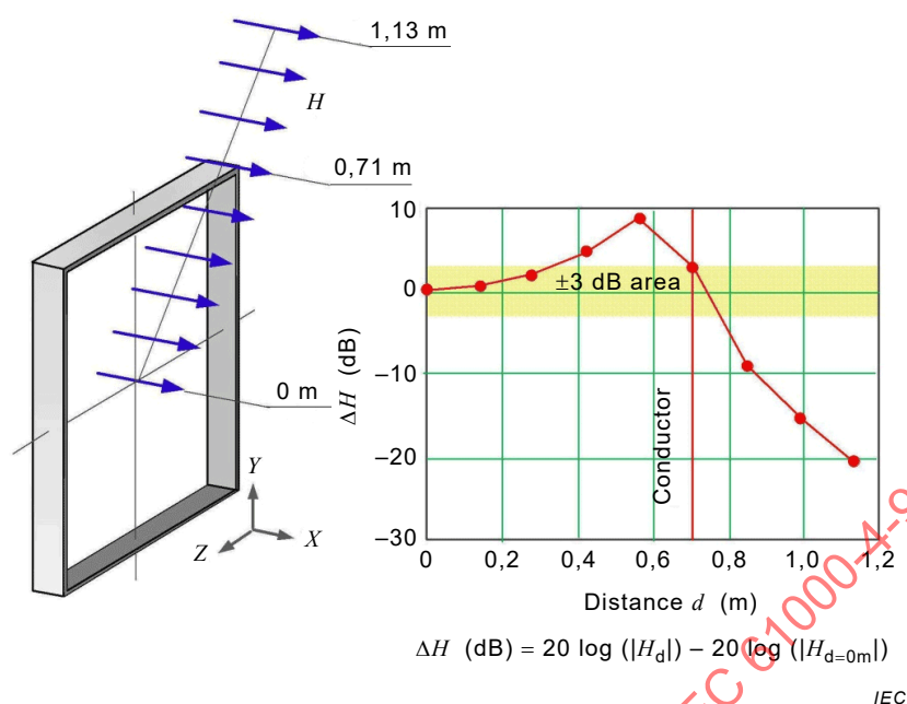
Figure G.5 – H_x -field along the diagonal in dB for the 1 m × 1 m induction coil
