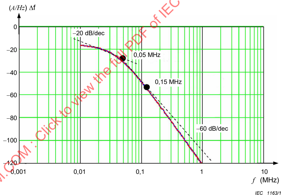
Figure E.6 – Courant de choc (8/20 \mu\text{s} ): réponse spectrale, \Delta f = 10 \text{ kHz}
