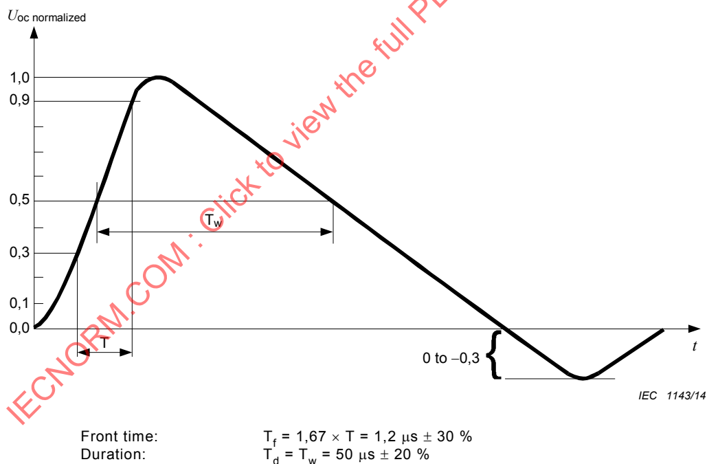
Figure 2 – Waveform of open-circuit voltage (1,2/50 \mu s) at the output of the generator with no CDN connected
