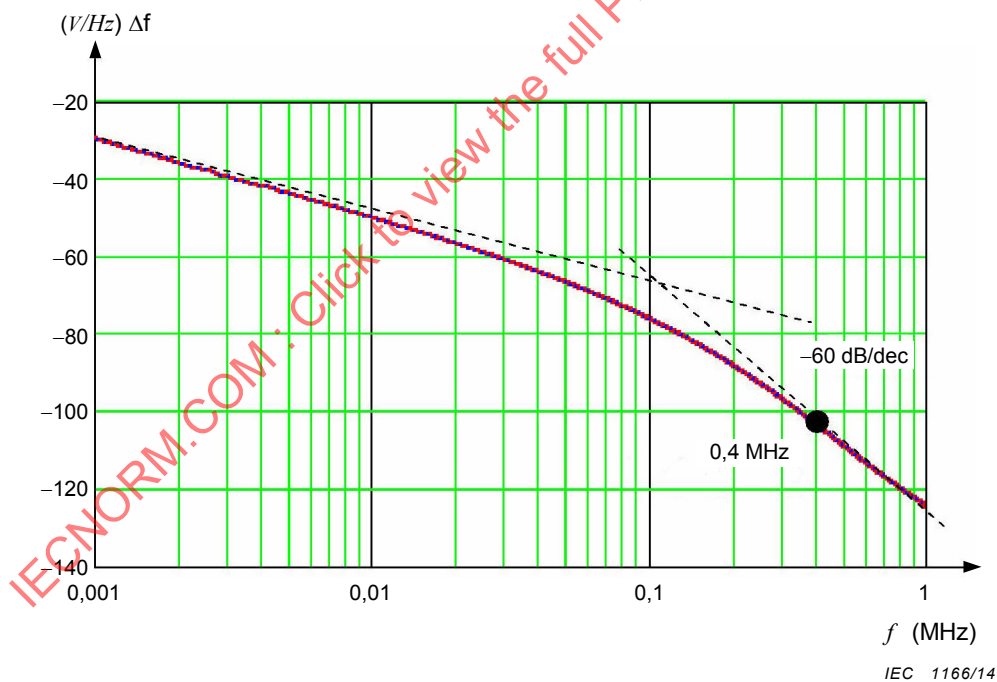
Figure E.9 – Voltage surge (10/700 \mu s): spectral response with \Delta f = 0,2 kHz
