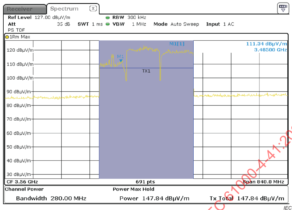
Figure D.1 – Example of a channel power measurement on a 5G spectrum
