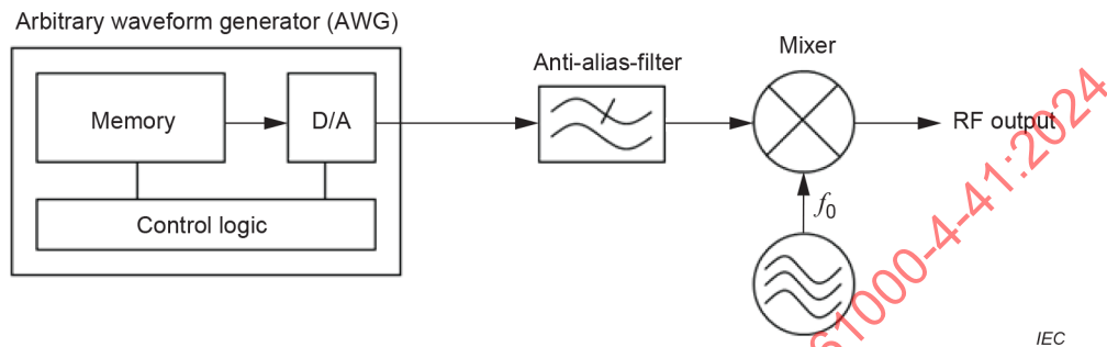
Figure A.3 – Principle of band-limited broadband signal generation with an arbitrary waveform generator
