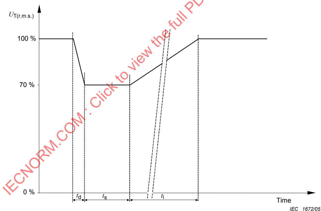
Figure 2 – Voltage variation
