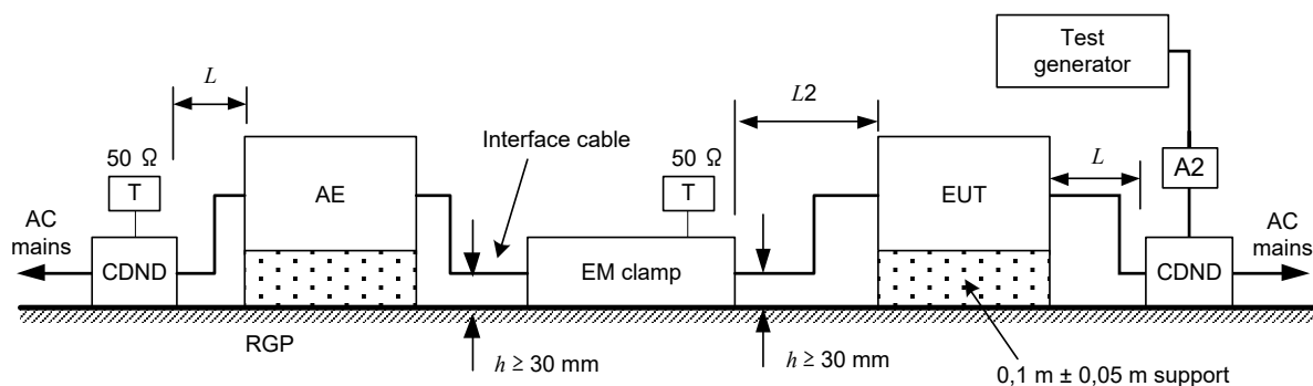
Figure 14b) – Schematic set-up when an AE shows errors during the test
