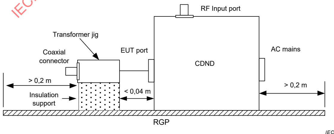
Figure 9 – Example of the set-up geometry to verify the insertion loss of the injection coupling system
