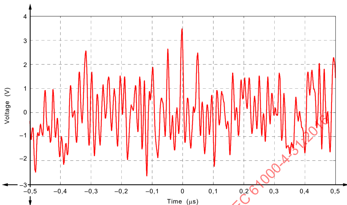
Figure B.4 – Extract of the band-limited pseudo noise signal in time domain (measured with an oscilloscope)
