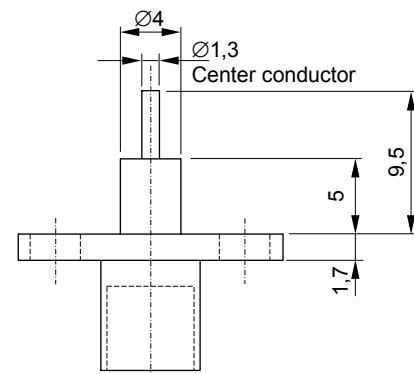
SMA-connector – Approximately 2:1
