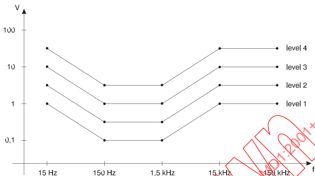
Figure 2 – Profile of the test voltage
