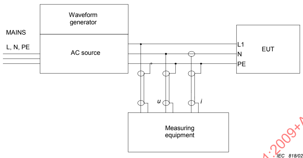
Figure 2 – An example of a test set-up for single phase
