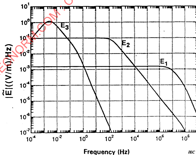
Figure 11 – Amplitude spectrum of each HEMP component
