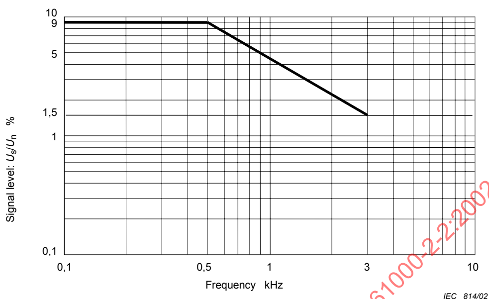
Figure 3 – Meister curve for ripple control systems in public networks (100 Hz to 3 000 Hz)
