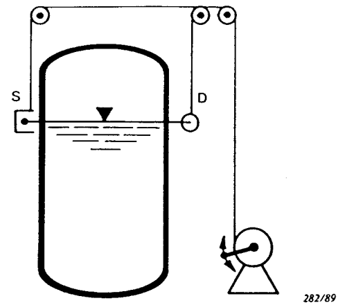
Figure 5 - Point source and point detector continuously following the level
