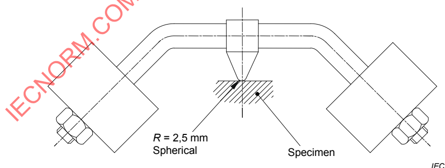
Figure 8 – Ball-pressure apparatus
