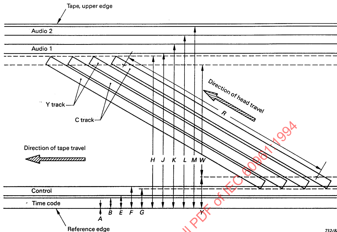
Figure 3 – Record locations and dimensions
