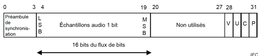
Figure 2 – Sous-trame audio 1 bit
