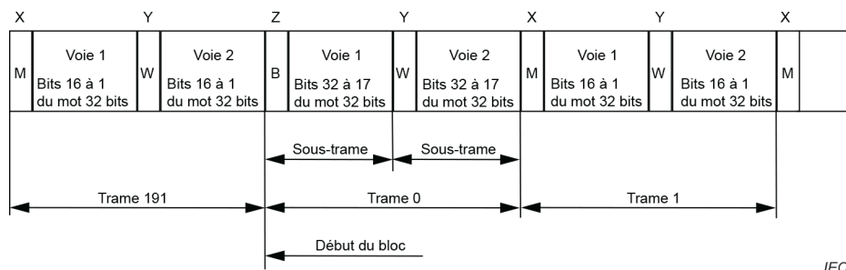
Figure 4 – Trame du mode 32 bits
