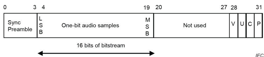
Figure 2 – One-bit audio subframe
