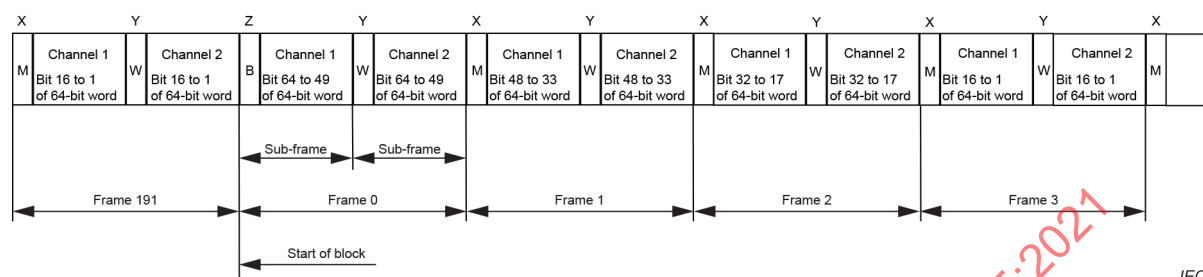
Figure 5 – 64-bit mode frame
