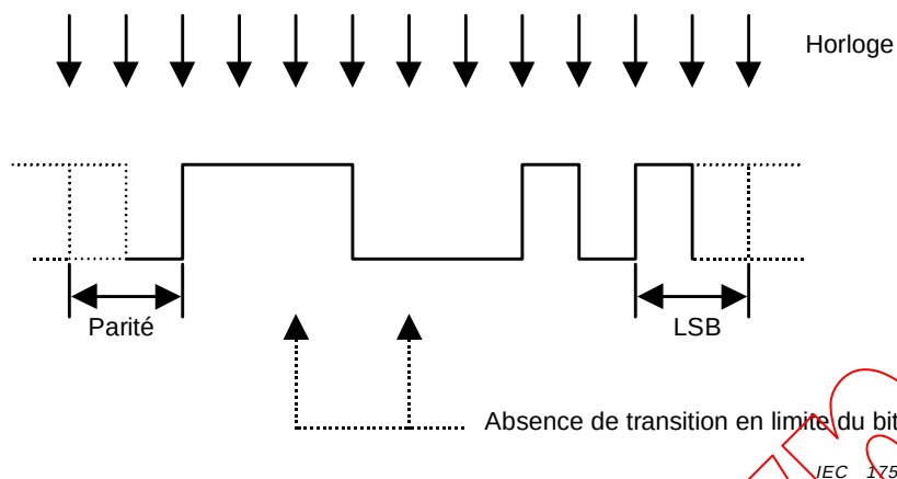
Figure 4 – Préambule M (11100010)
