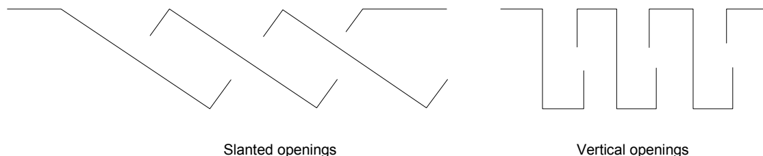
Figure 4B – Examples of cross-sections of designs of openings preventing vertical access
