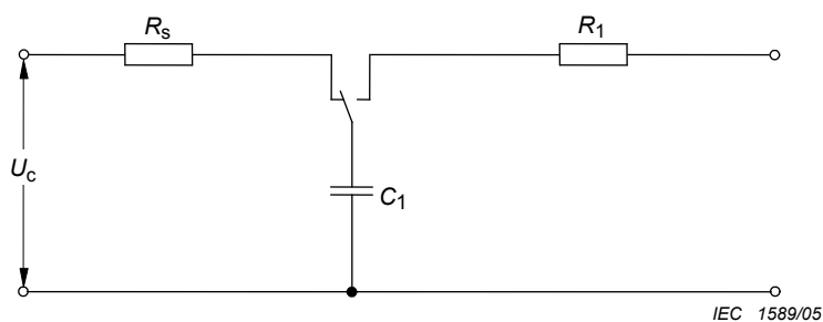
Figure N.2 – IEC 60065 impulse test generator circuit
