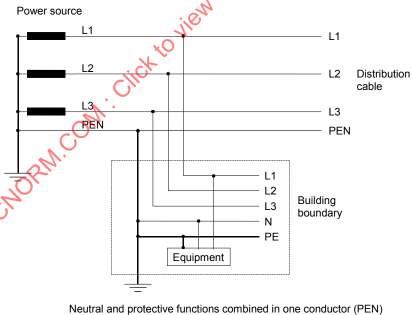
Figure V.2 – Example of TN-C-S power distribution system
