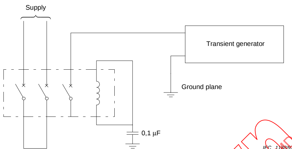
Figure 4 – Test circuit for the verification of the influence of transients in the main circuit (common mode)
