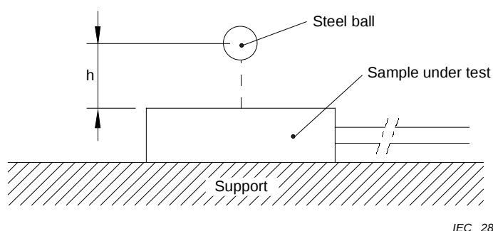
Figure B.2 – Test device
