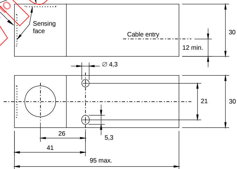
Figure A.1.3 (IC) – Dimensions in millimetres
