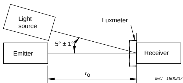
Figure 11a – Type T, emitter and receiver
