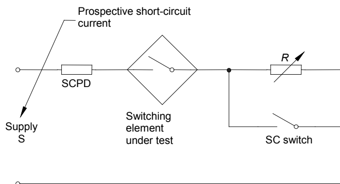
Figure H.3 – Short-circuit testing (see H.8.6.1)
