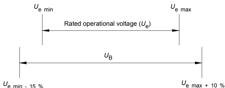
Figure H.1 – Relationship between U_e and U_B
