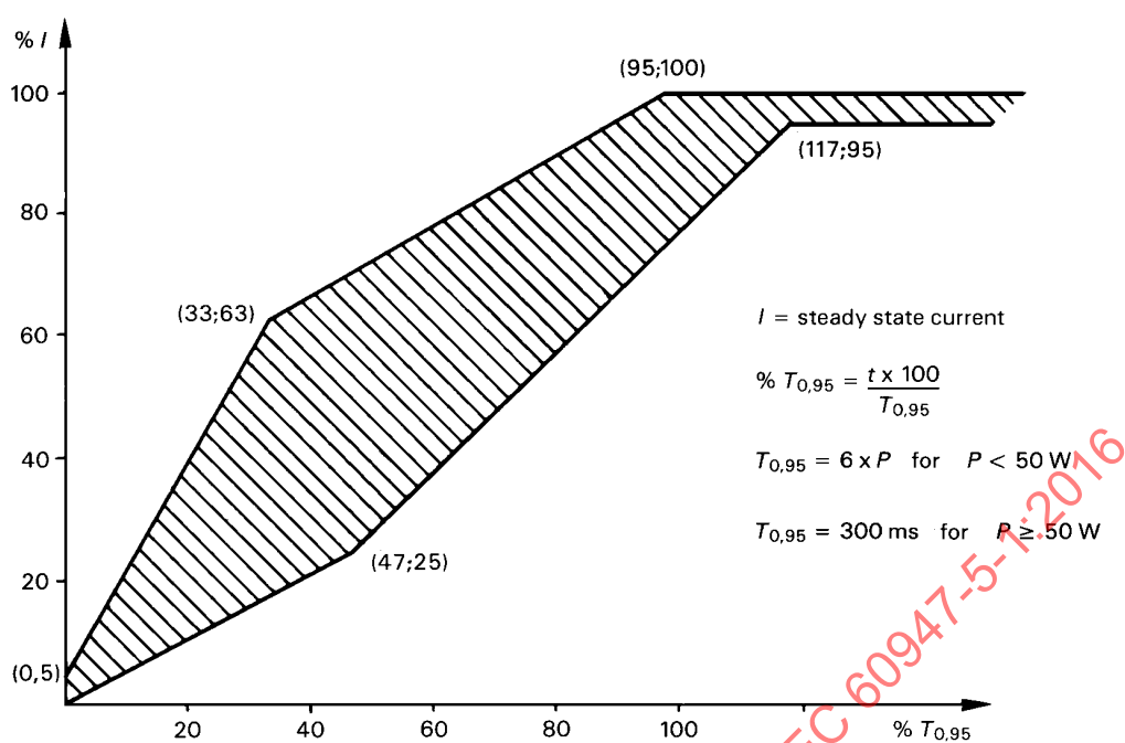
Figure 9 – Current/time limits for d.c. test loads (see 8.3.3.5.4)
