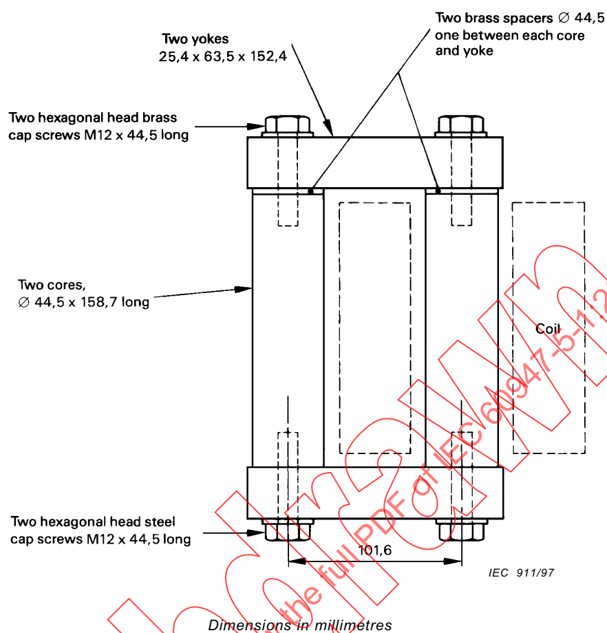
Figure B.1 – Construction of load for d.c. contacts
