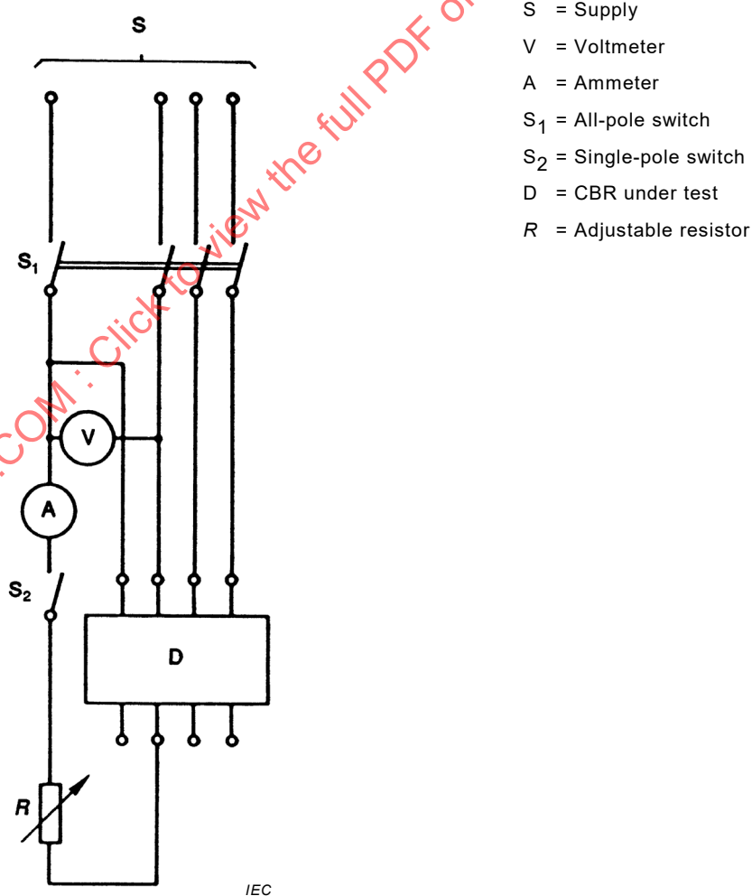
Figure B.1 – Test circuit for the verification of the operating characteristic (see B.8.2)
