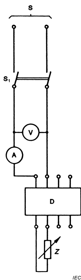
Figure B.2 – Test circuit for the verification of the limiting value of the non-operating current under over-current conditions (see B.8.5)
