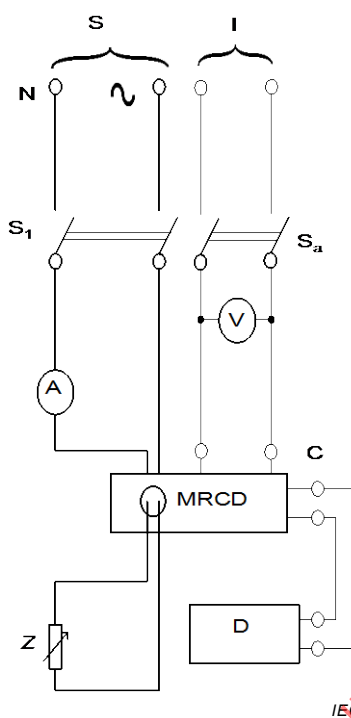
Figure M.4b) – MRCD with integral sensing means
